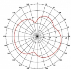
Far-field amplitude of Cable-20cm-E.nsi
