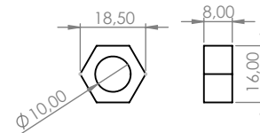
M10 Hexagonal nut
