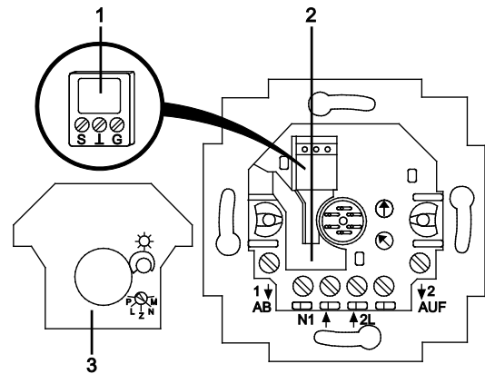
Fig. 9: Connecting the sensor
