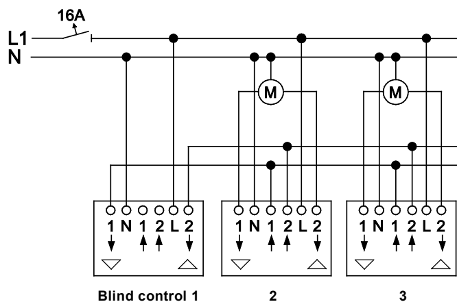
Fig. 7: Group control
