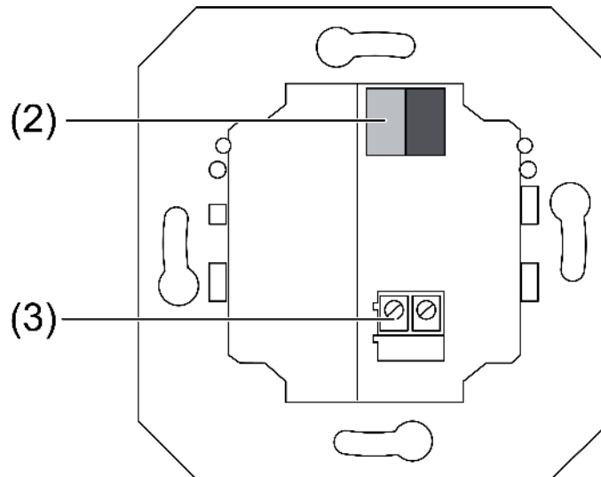
Figure 2: Rear side
