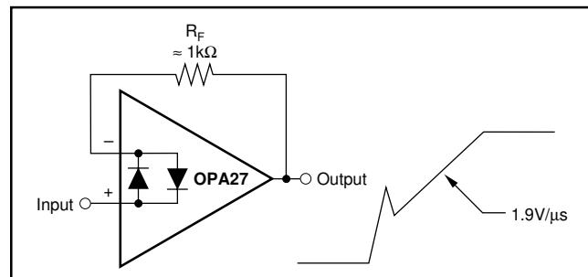
FIGURE 6. Pulsed Operation.
