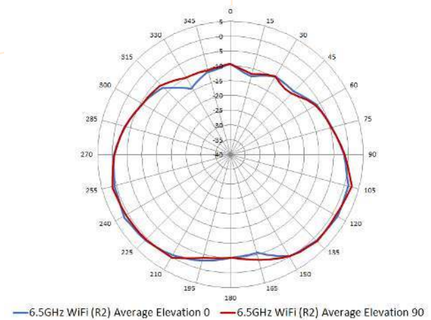
6.5GHz Wi-Fi antennas patterns (vertical)
