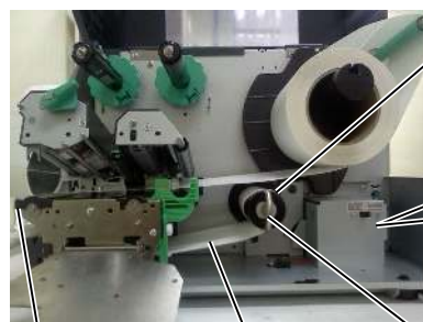
Strip Plate
