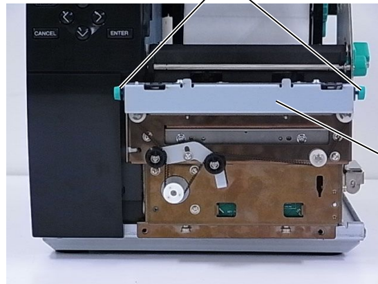
Cutter Unit
